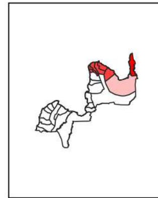
TROPICAL CYCLONE
