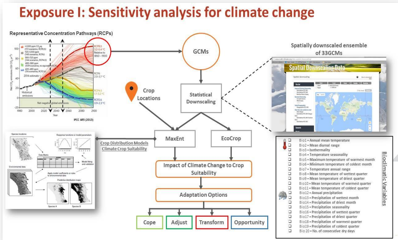
Figure 4. Sensitivity Analysis for Climate Change
